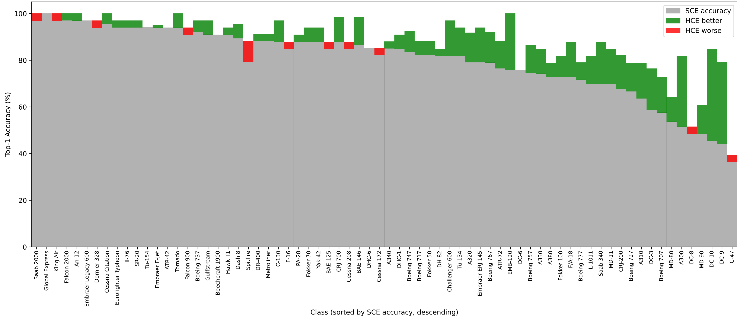
ResNet-50 — Per-family accuracy: SCE vs HCE
